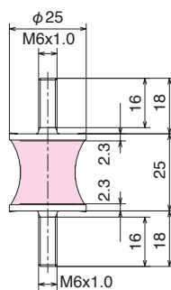
KXA-25-25H
