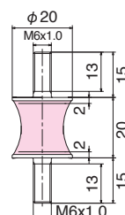
KXA-20-20H
