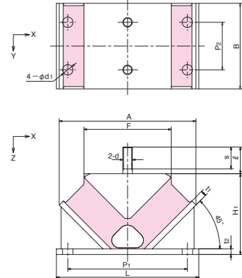
■ KC-140BP~170BP
